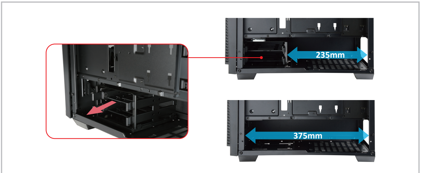
Removable HDD Cage Creates Flexible Space for PSU Cable Routing
